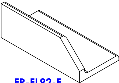
FP-FL92-F FENDER FLARE ANGLE, FL92, AI 1-1/2 x 2 x 1/4
