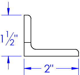
FP-FL92-F FENDER FLARE ANGLE, FL92, AI 1-1/2 x 2 x 1/4
