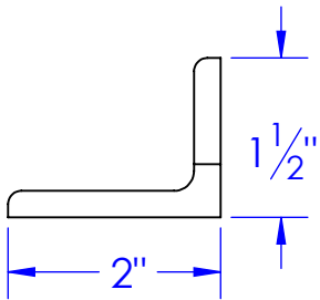
FP-FL92-E FENDER FLARE ANGLE, FL92, AI 1-1/2 x 2 x 1/4
